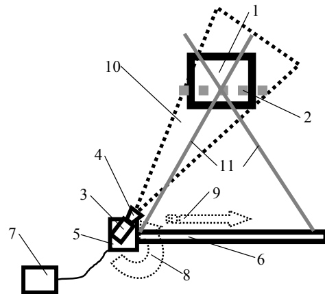
Fig. 2 A diagram of the HoloCam system - 1. The object to be recorded; 2. Future hologram image plane; 3. Digital camera at the left-most position at the electromechanical stepper-motor rail; 4. Camera zoom objective; 5. Stepper-motor precision rotation stage; 6. Electromechanical stepper-motor rail; 7. Rotation stage and translation rail controller; 8. Digital camera angular movement; 9. Digital camera linear movement; 10. FOV of the digital camera; 11. two laser pointers beam.
